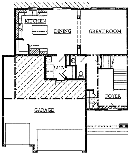
MAIN LEVEL 977 SQ.FT.
