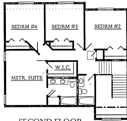
SECOND FLOOR 1050 SQ.FT.
