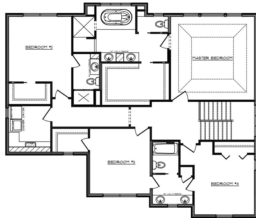
SECOND FLOOR SQ. FT. - 1646
