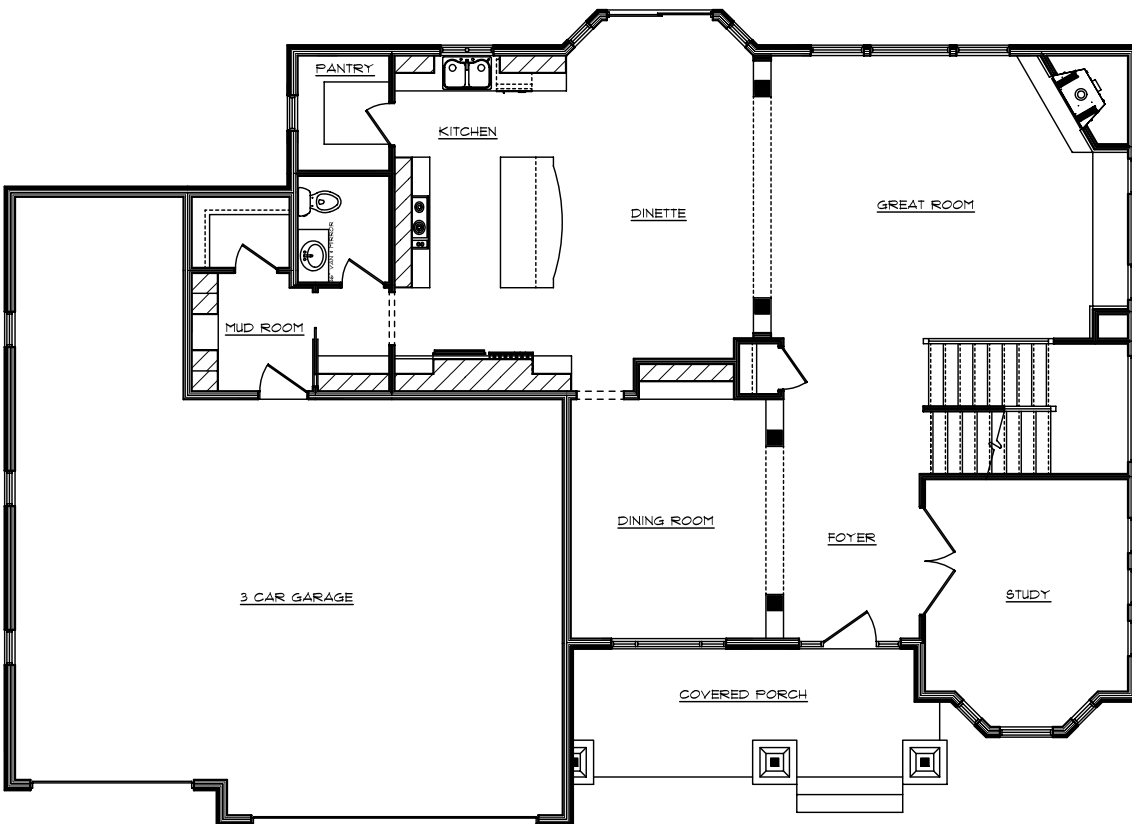
MAIN FLOOR SQ. FT. - 1483
